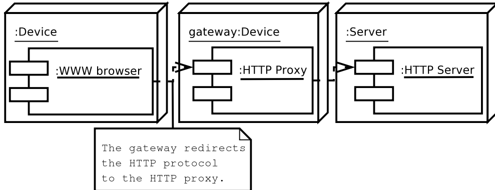
Figure 2.9: Transparent proxy.
