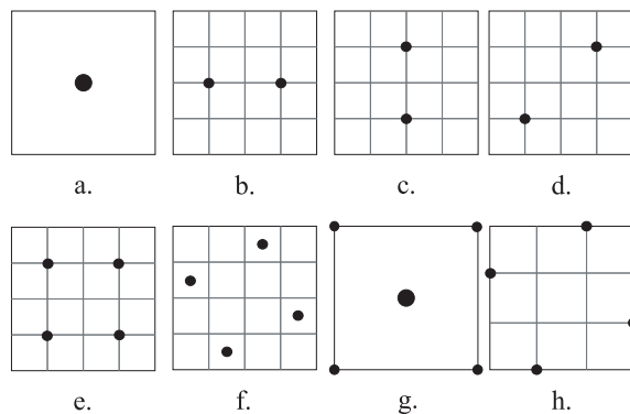
Figure 1: A collection of sampling schemes. From top left to bottom right: a) Centroid sampling, b) Kyro horizontal, c) Kyro vertical, d) Diagonal, e) 2 \times 2 box pattern, f) Rotated Grid Supersampling (RGSS), g) Quincunx, h) FLIPQUAD.
